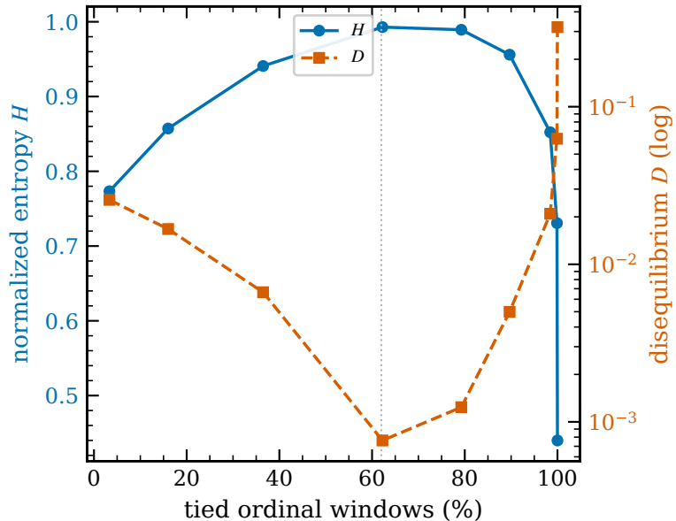
(b) Quantization moves the plane non-monotonically
