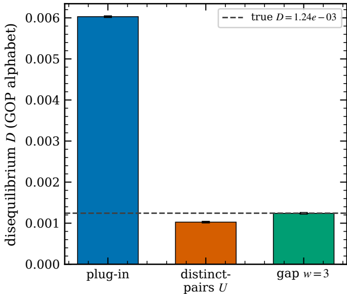
(a) Overlap bias ports to ties ( m=4 , M=75 , N=200 )
