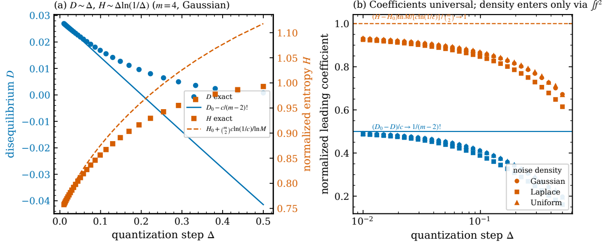
Fig. 1: Leading-order discretization law. (a) For Gaussian white noise the disequilibrium D follows the linear law D_0 - c/(m-2)! while the entropy follows H_0 + \binom{m}{2} c \log(1/c) / \log M , with c(\Delta) = \sum_k q_k^2 the per-pair coincidence probability. (b) Normalizing by c , the leading coefficients converge to 1/(m-2)! and \binom{m}{2} for Gaussian, Laplace and uniform sources: the coefficients are universal and the source density enters only through \int f^2 .
