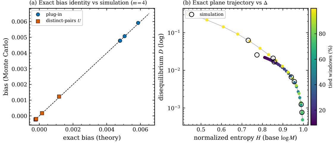
Fig. 2: The exact plane trajectory as the quantization step grows. The tie-aware coordinates trace a non-monotonic path: the maximally random continuous process is not at maximum entropy on the tie alphabet, and coarser quantization first raises the apparent entropy by activating tie patterns. Open circles: direct simulation; filled points: the exact theory of Sec. 4.
