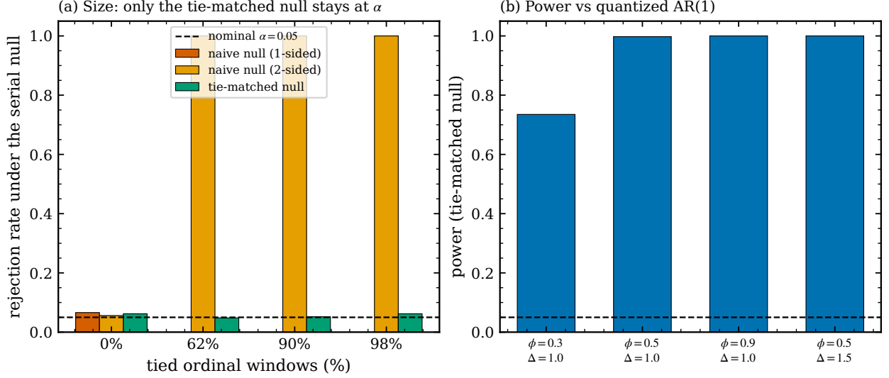
Fig. 3: Calibrated inference on quantized data. (a) Under a true IID (but quantized) process the tie-matched permutation null holds size at the nominal \alpha = 0.05 across tie fractions, while the tie-free null does not: two-sided it rejects every series. (b) Power of the tie-matched null against quantized AR(1).
