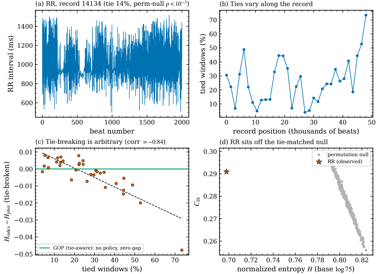
Fig. 4: Interbeat-interval record 14134 (integer samples). (a) A representative window. (b) Tie fraction along the record. (c) The conventional tie-broken plane is policy-dependent: the signed index–jitter entropy gap grows with the tie fraction (correlation -0.84 ), while the tie-aware treatment needs no policy. (d) On the tie alphabet the observed series sits off its own tie-matched permutation null, confirming genuine serial structure.
