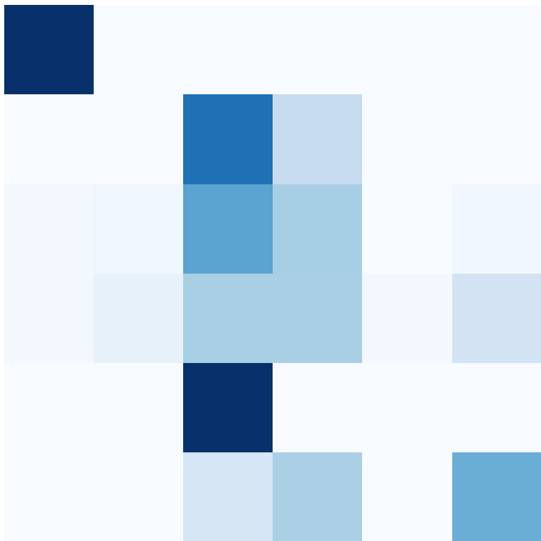
Opportunity: Qwen3-0.6B
