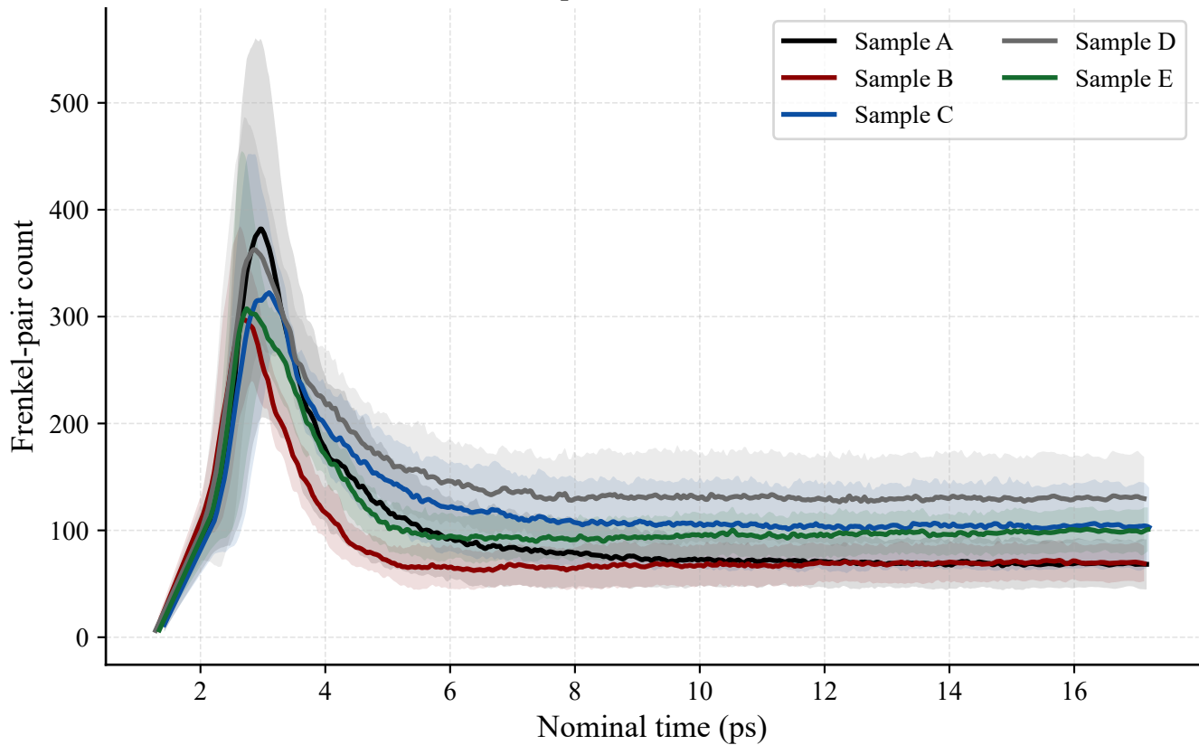
Frenkel-pair evolution at 5 keV
