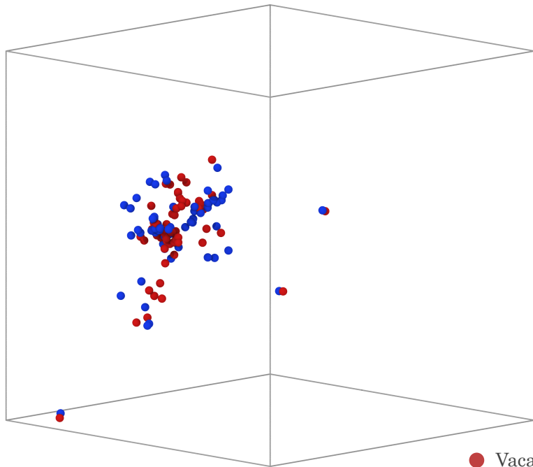
Sample A Frenkel pairs - 63
