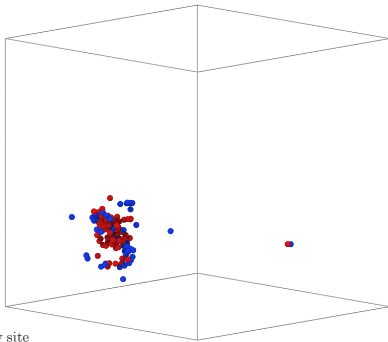
Sample B Frenkel pairs - 72
