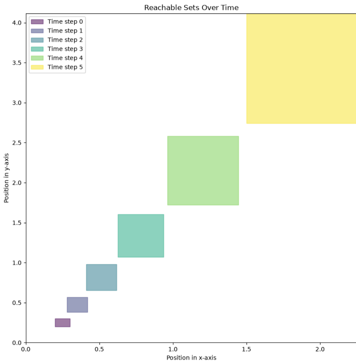
Figure 1: Reachable sets using interval matrix method up to T = 5
