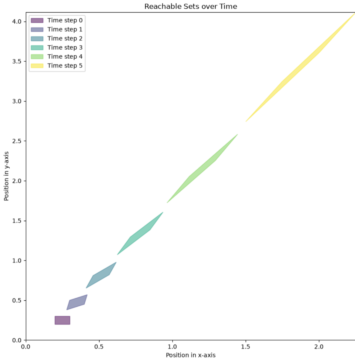
Figure 3: Reachable sets using vertex shooting method up to T = 5
