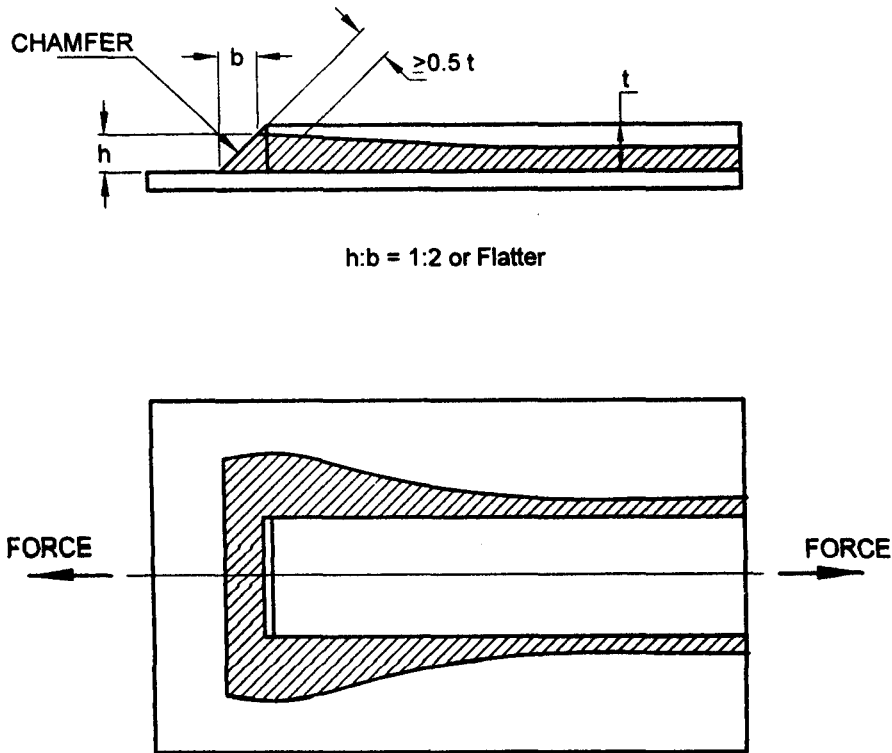
FIG. 19 END FILLET WELD NORMAL TO DIRECTION OR FORCE
