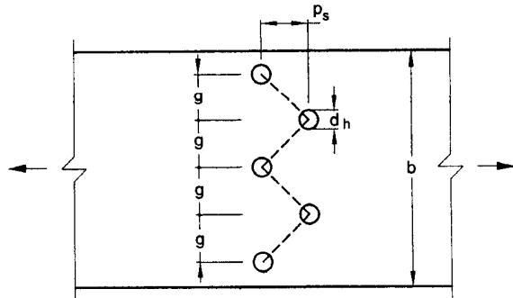
FIG. 5 PLATES WITH BOLTS HOLES IN TENSION
