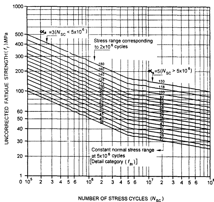
FIG. 22 S-N CURVE FOR NORMAL STRESS
