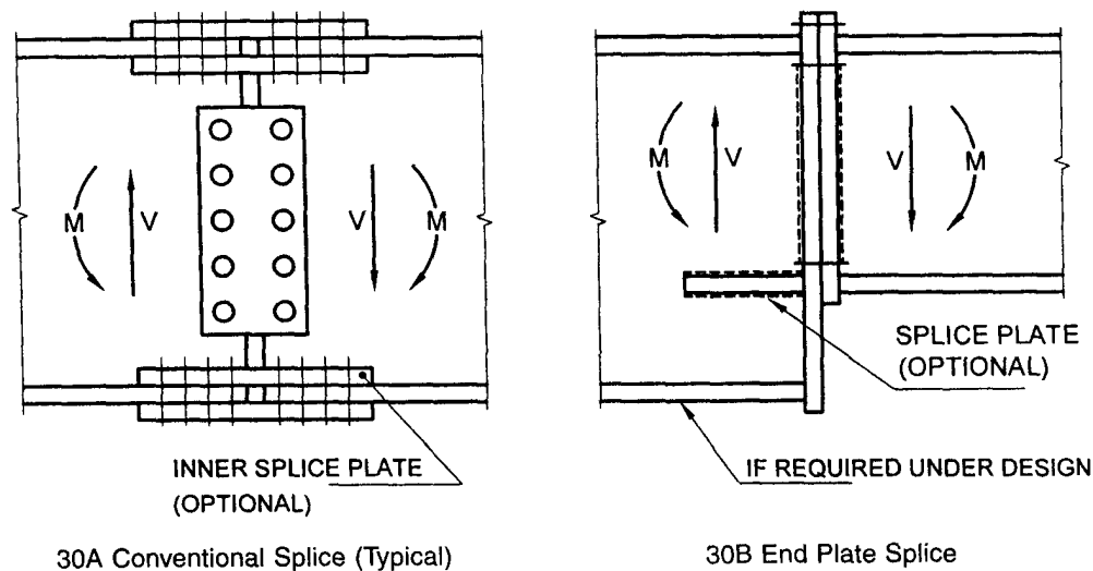
FIG. 30 BEAM SPLICES
