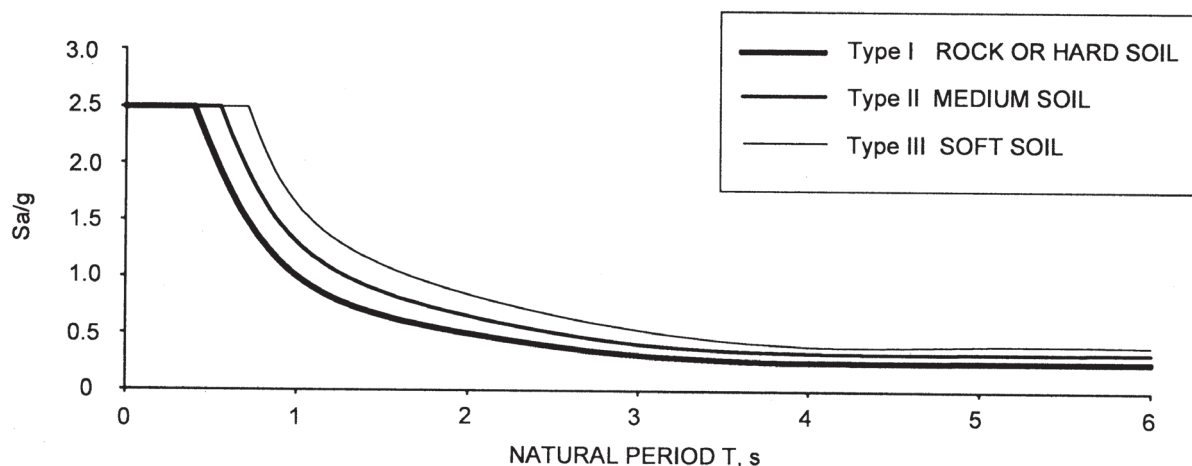
2A SPECTRA FOR EQUIVALENT STATIC METHOD
