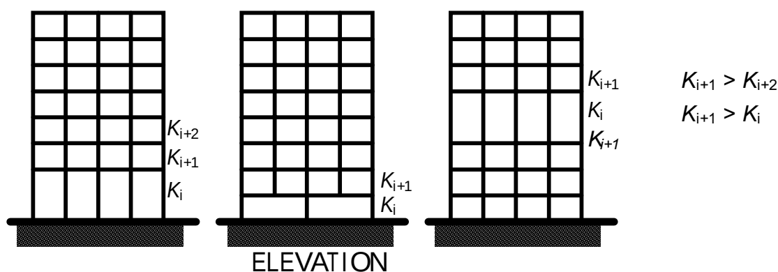
4A STIFFNESS IRREGULARITY (SOFT STOREY)
