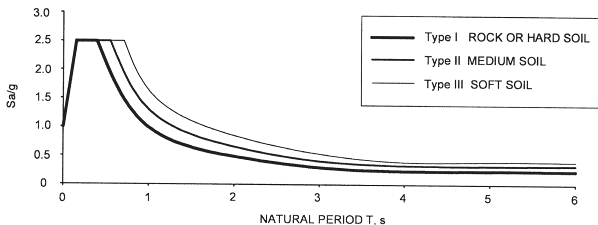
2B SPECTRA FOR RESPONSE SPECTRUM METHOD
