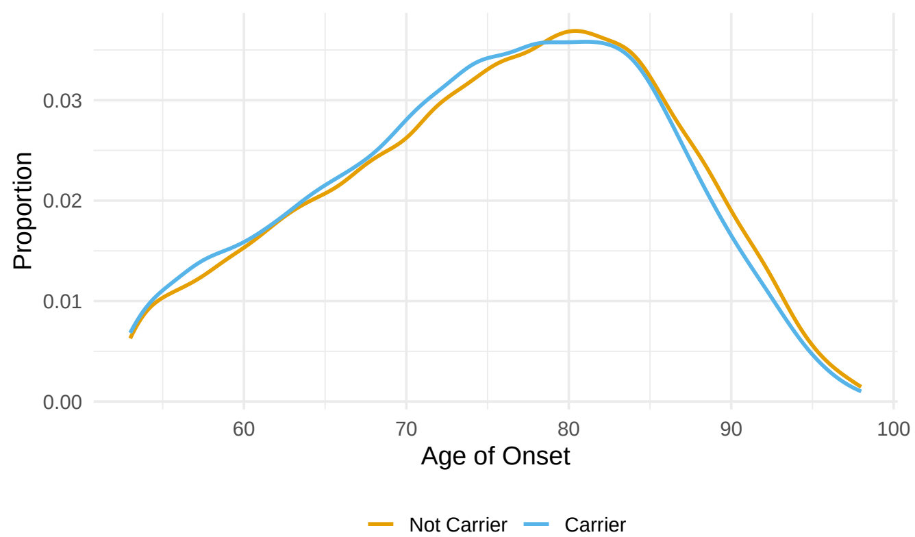
(F) APOE4 Carrier Status
