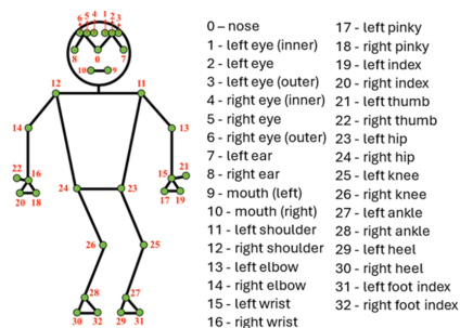
Gambar 2.2 Diagram 33 Landmark MediaPipe Pose
