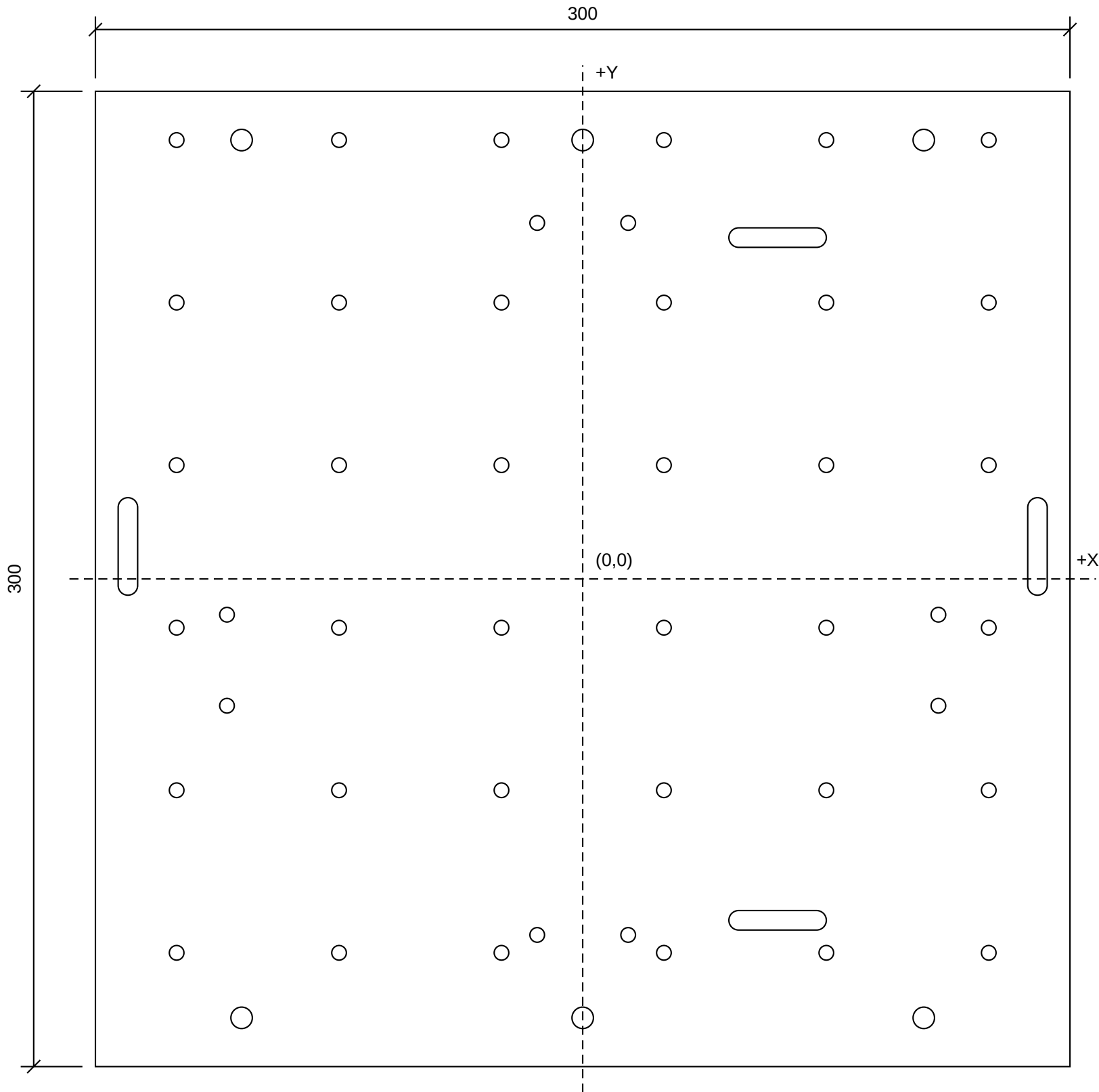
TOP VIEW | Origin at plate centre | 50mm pitch; X edge25, Y first35 / last15 (grid Y offset+10)
