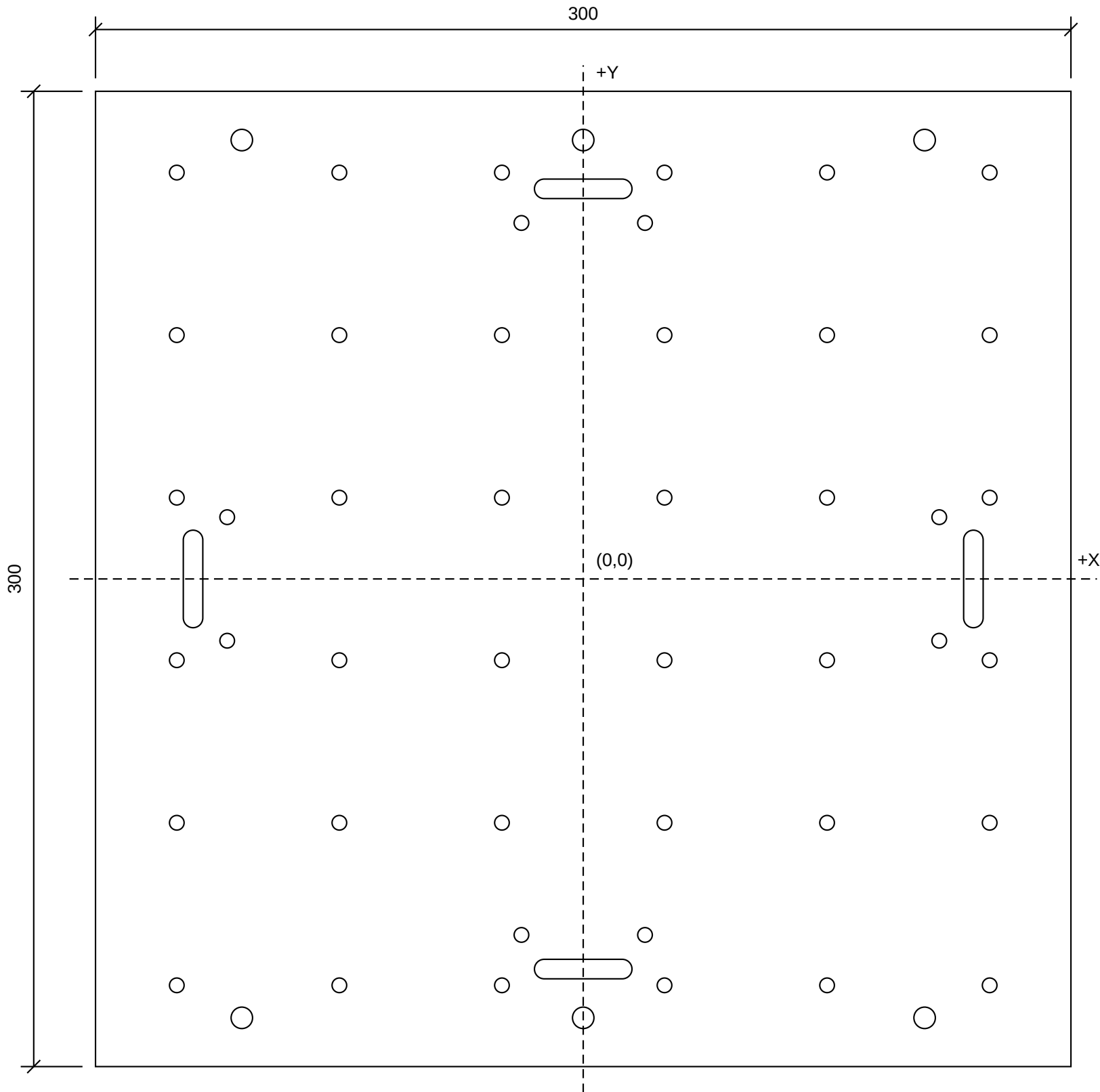
TOP VIEW | Origin at plate centre | Grid edge offset 25, pitch 50 (both axes)
