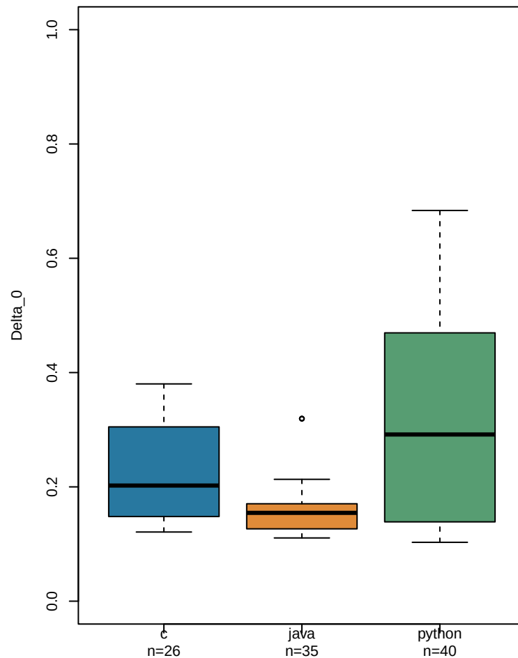
Token sequence
