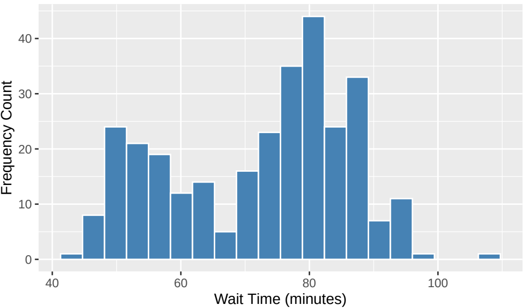
Distribution of Time Between Eruptions
