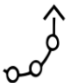
S21f17 IOU=0.54
