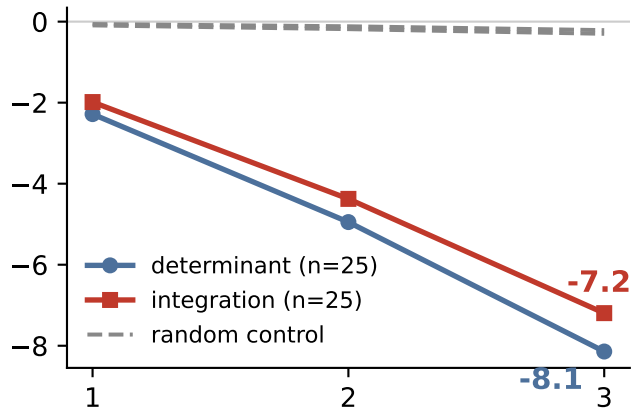
Qwen2.5-72B — steer L75+L78 MLP
