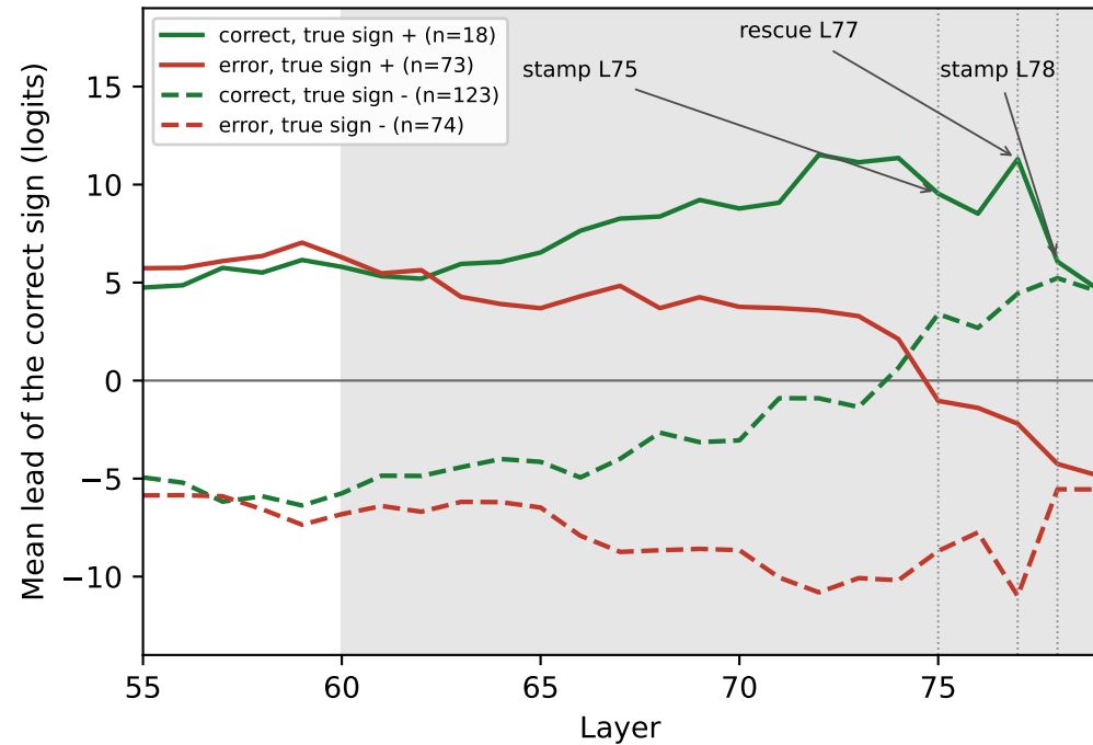
Qwen2.5-72B
