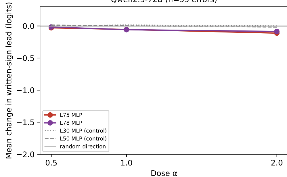
Qwen2.5-72B (n=99 errors)
