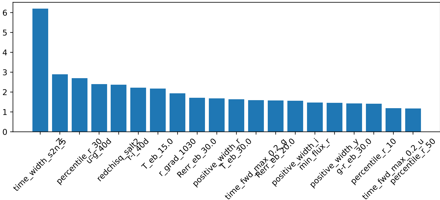
Feature Importances
