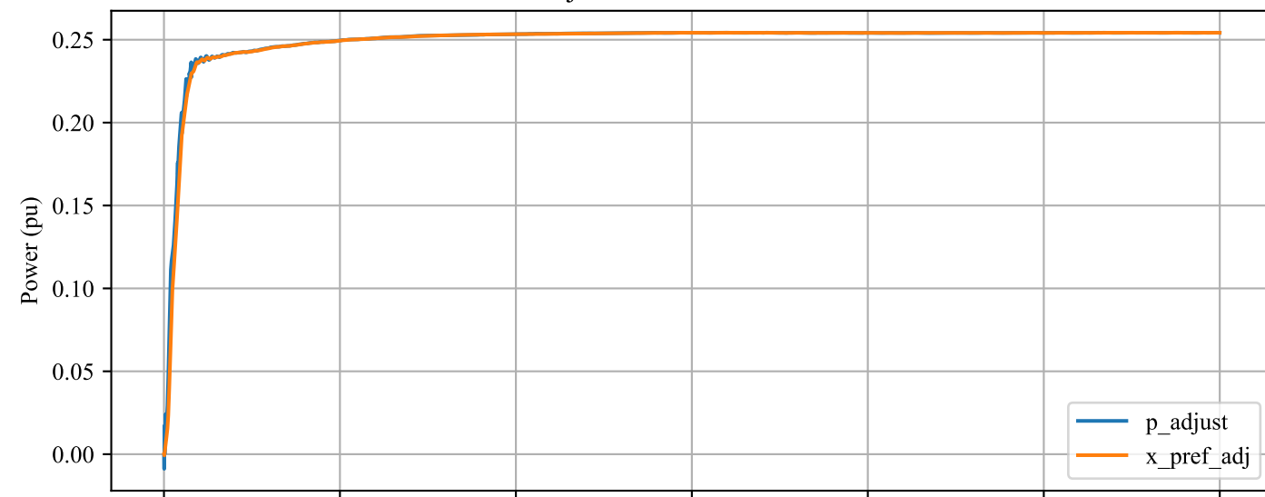
GSC Power Reference
