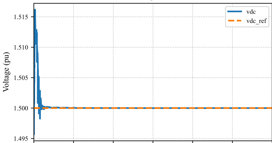
DC Voltage Controller Power Adjustment
