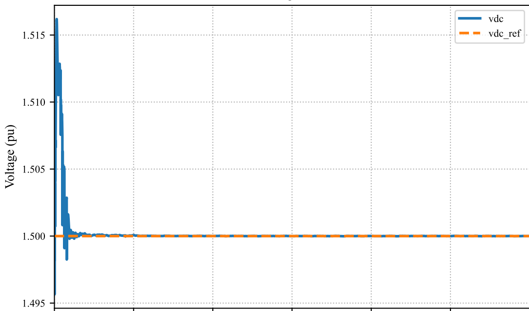
DC-link Voltage vs Reference
