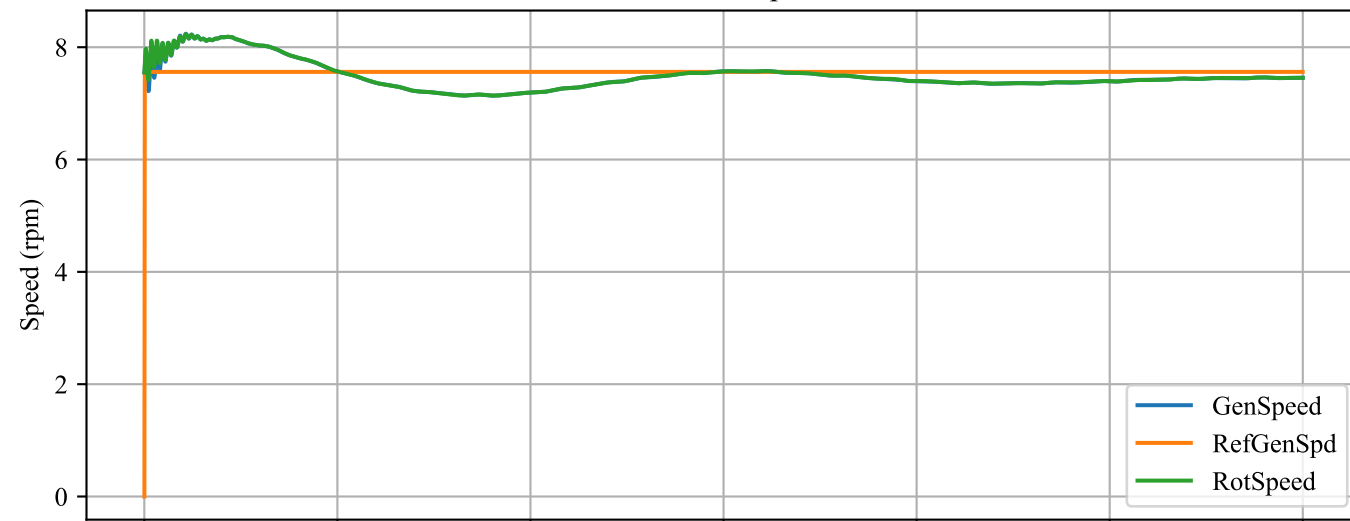
Generator Speed
