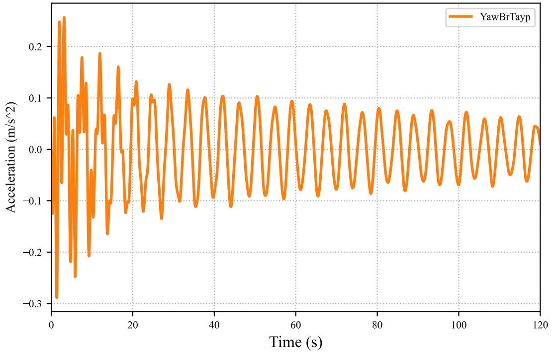
Yaw Bearing (tower top) Translational Acceleration Y-axis
