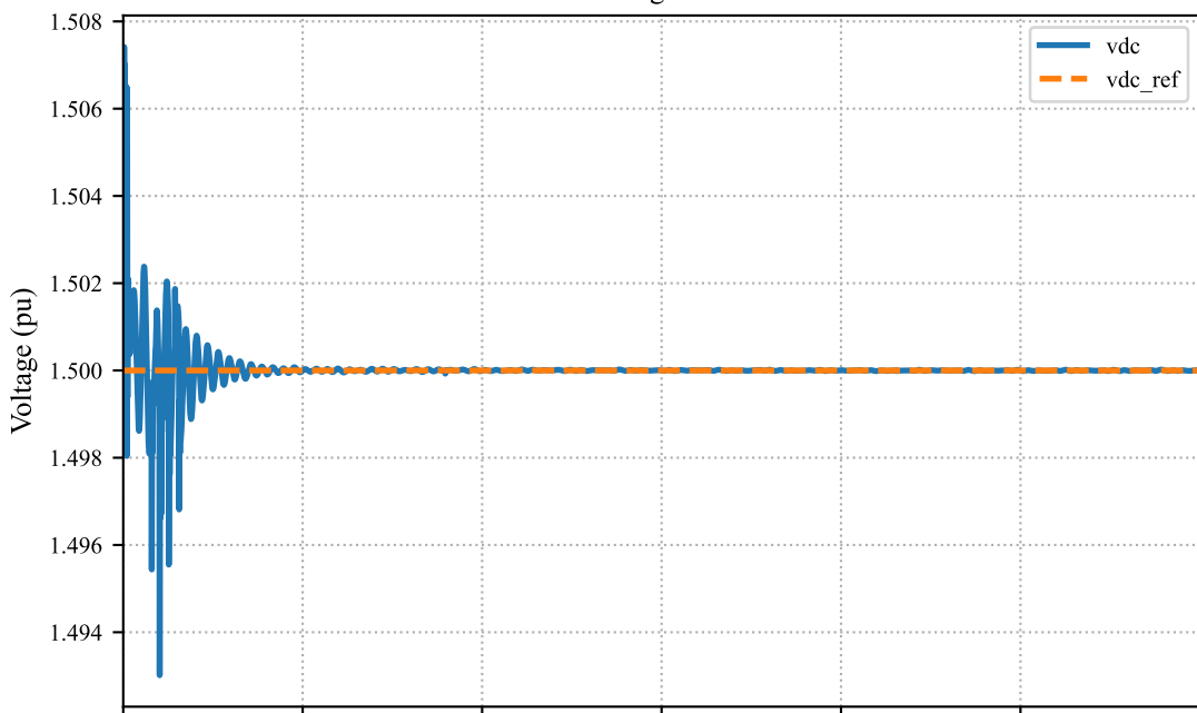
DC Voltage Controller Power Adjustment
