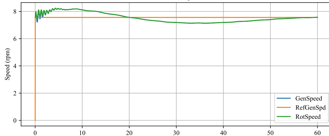
Generator Speed
