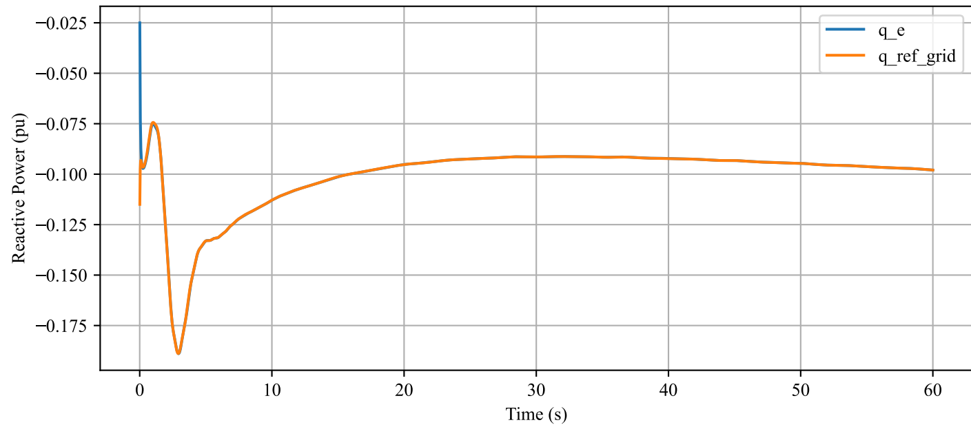
Reactive Power
