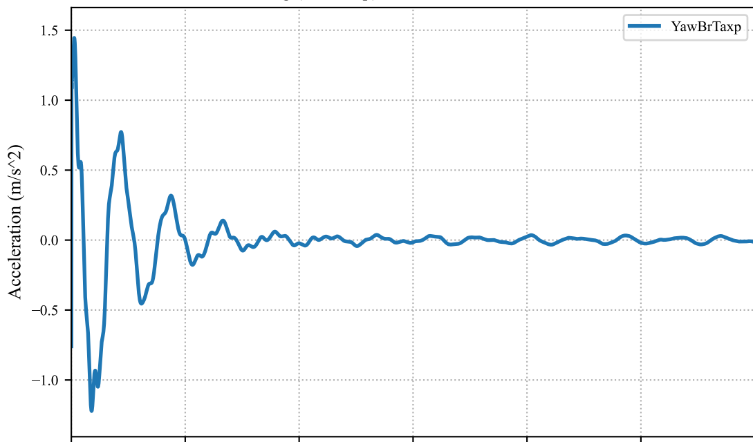
Yaw Bearing (tower top) Translational Acceleration Y-axis
