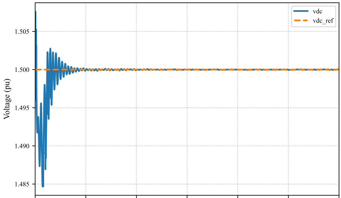
DC Voltage Controller Power Adjustment
