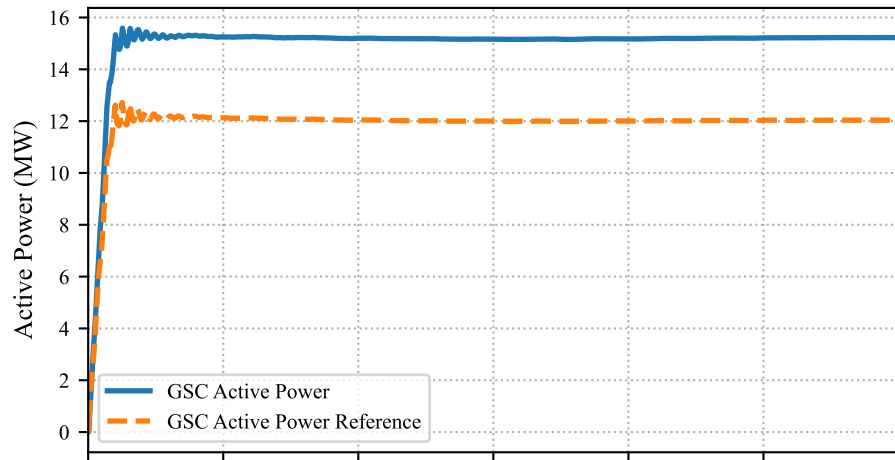
Generators Active Power Injections
