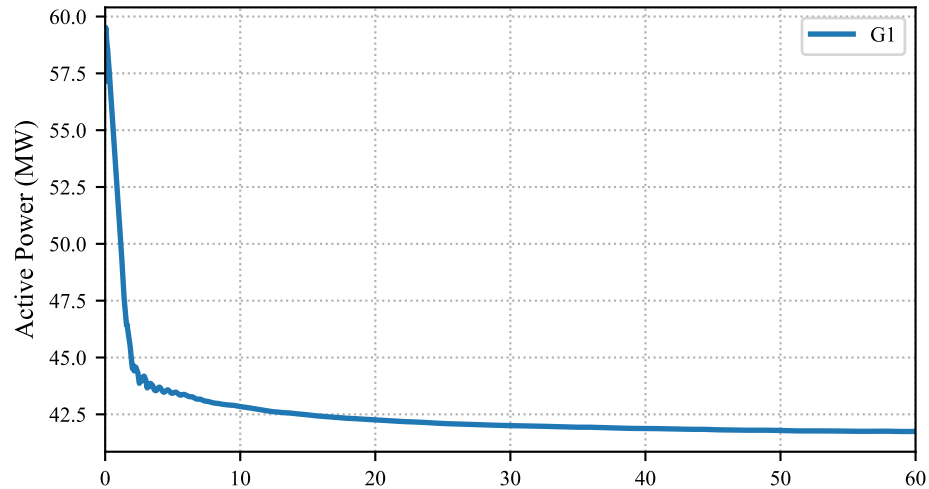
Generators Active Power Injections
