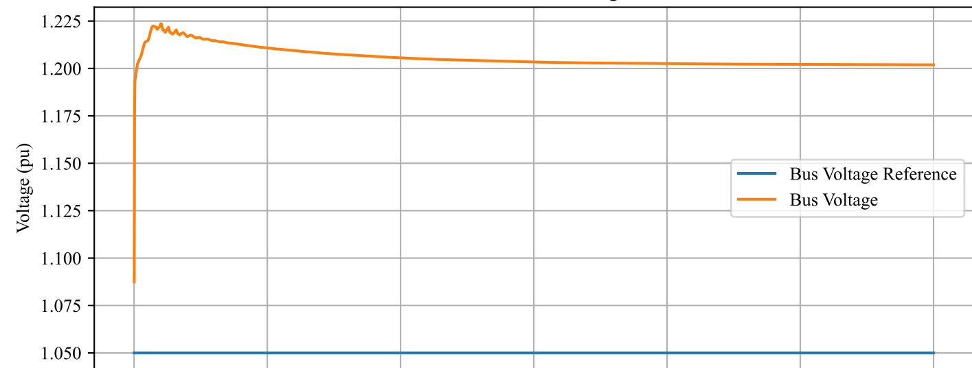
Bus Terminal Voltage
