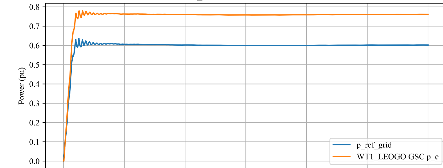
WT1_LEOGO GSC Active Power
