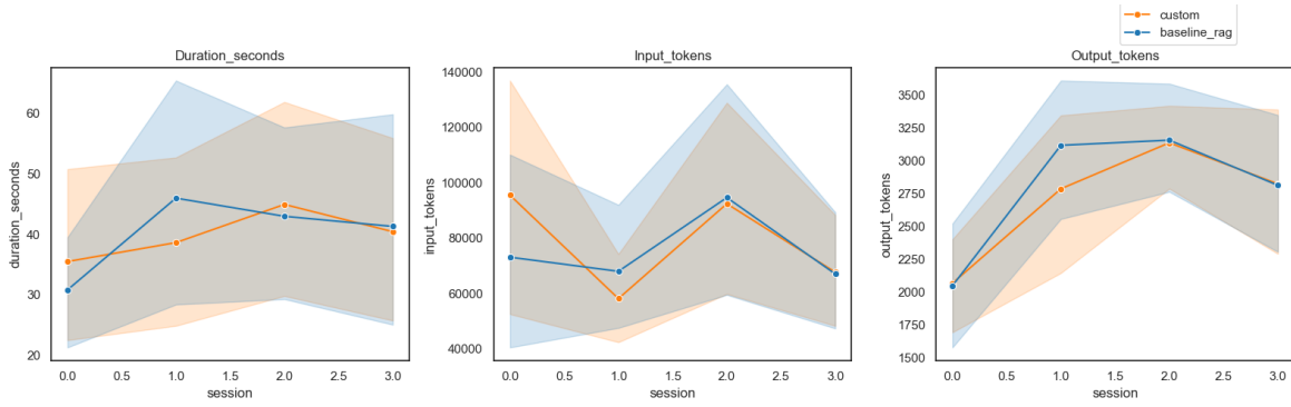
Figure 4.12: Resource metrics across sessions. Token counts and latencies fluctuate without a systematic trend for either configuration, and the two track each other throughout.
