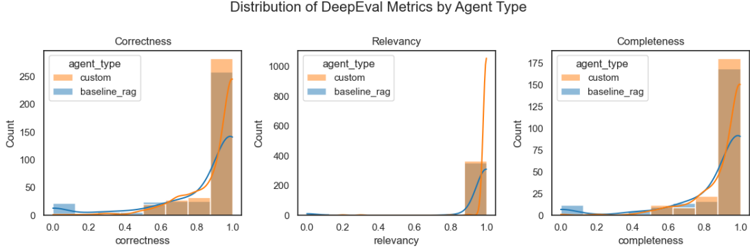
Figure 3.5: Distribution of DeepEval metric scores across all queries, agents, and sessions. The pronounced left-skew and heavy concentration near 1.0 violate the normality assumption, motivating the use of non-parametric Mann-Whitney U tests for all comparisons.
