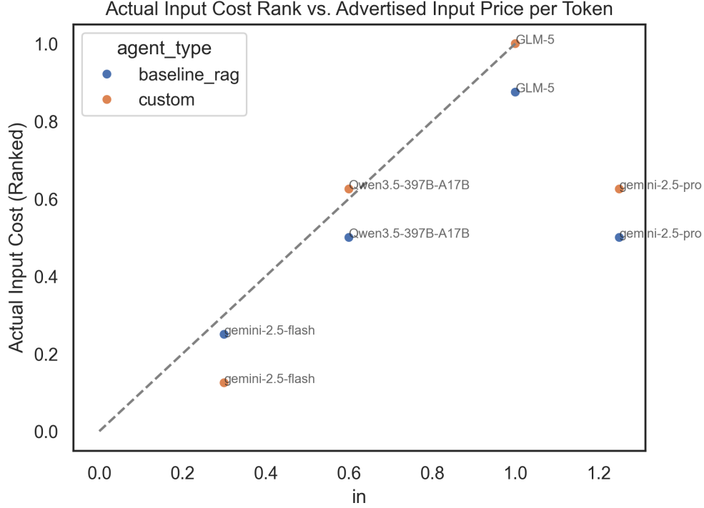
Figure 4.17: Actual input cost (ranked) vs. advertised input price per token. The diagonal reference line represents perfect proportionality — if advertised price fully predicted actual cost, all points would lie on this line. The non-linear deviation indicates that more capable models can be more token-efficient.
