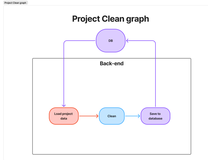
Figure 3.4: Clean pipeline graph: load_project \rightarrow clean \rightarrow save_results , used for both element deduplication and metadata rewriting.
