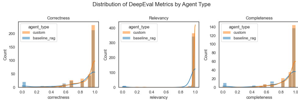
Figure 4.6: Aggregate distribution of all DeepEval metric scores. The custom agent’s distribution is more concentrated near the upper end, while the baseline exhibits a heavier low-scoring tail.
