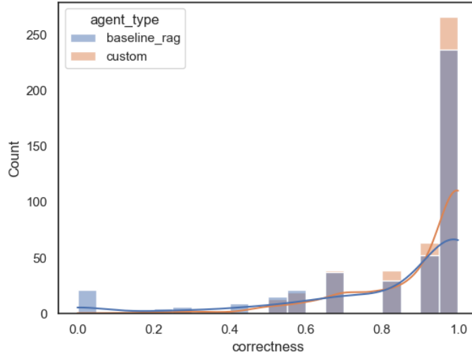
Figure 3.4: Distribution of correctness scores across all queries and sessions. The pronounced right-skew and heavy concentration near 1.0 violate the normality assumption, motivating the use of non-parametric Mann-Whitney U tests.
