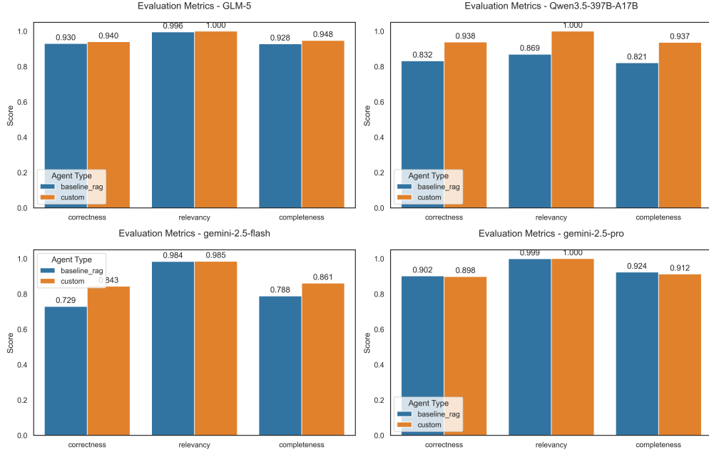
Figure 4.4: Metrics across models
