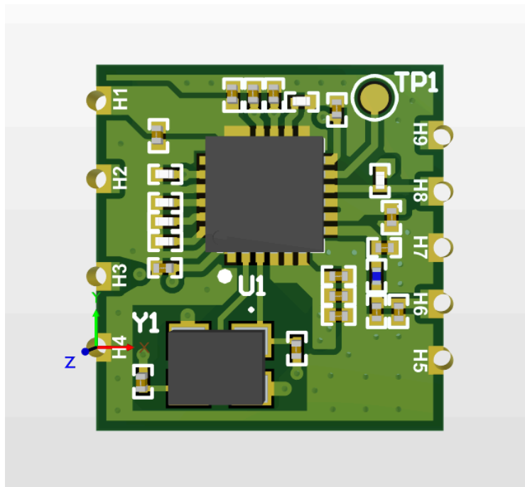
Fig 2(a) : Module Diagram (top view)
