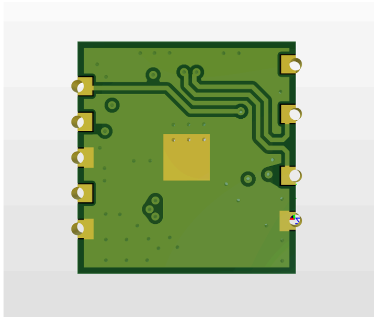
Fig 2(b) : Module Diagram (Bottom view)
