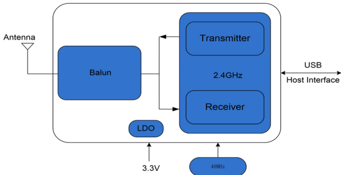
Fig 5 : Block Diagram
