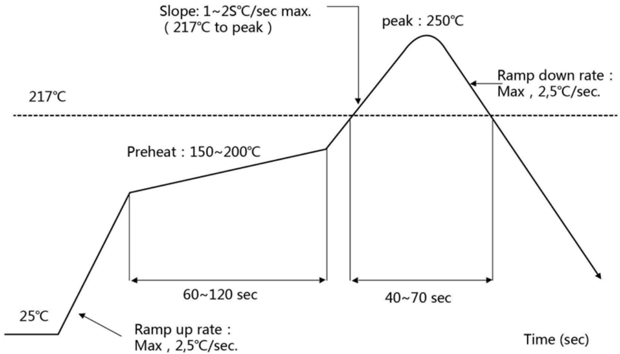
Fig 6 : Recommended Reflow Profile
