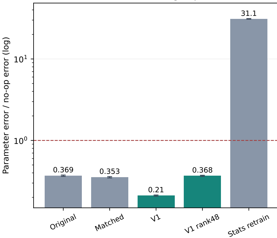
DS-Air: retained ridge optimum
