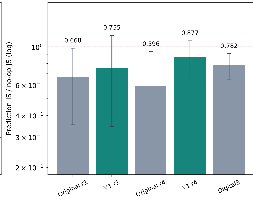
RTD-Air: independent-teacher KD
