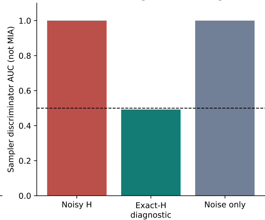
Randomized retraining remains distinguishable
