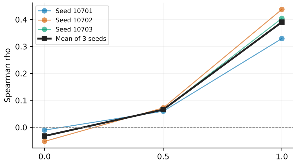
Achieved data-channel association
