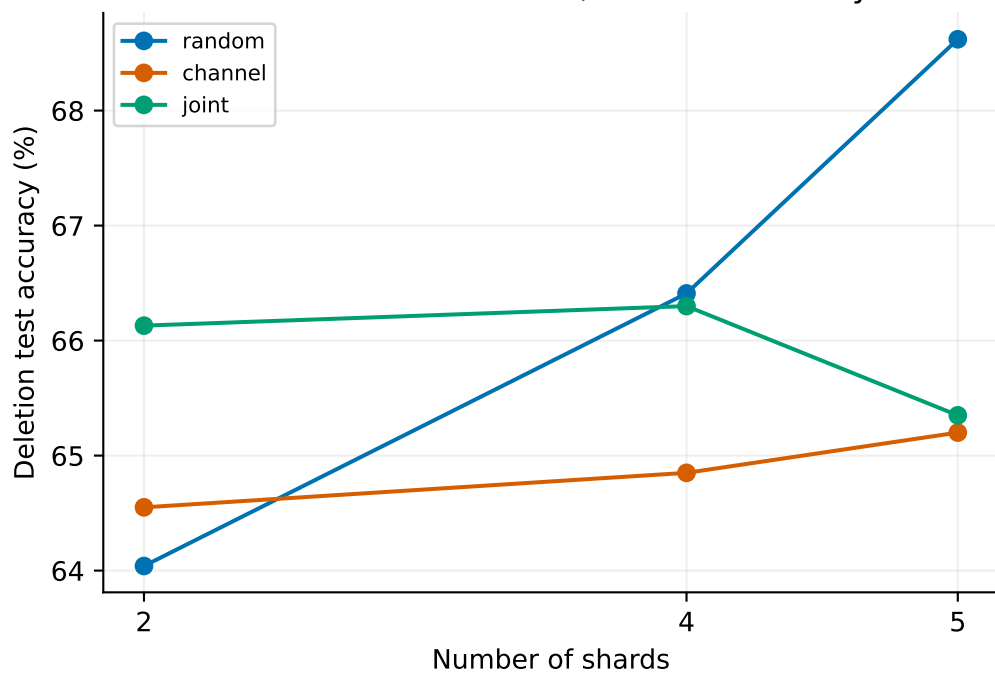
Shard count: SNR=10, screen seed only
