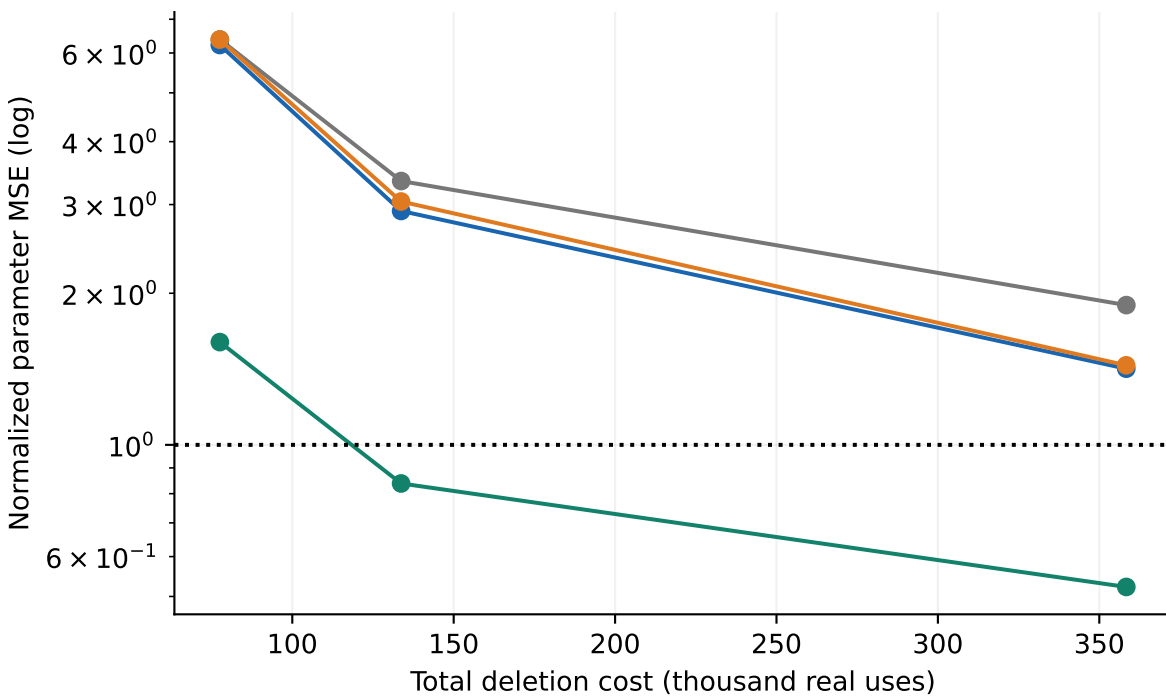
Curvature cost: FashionMNIST, D64, 20dB
