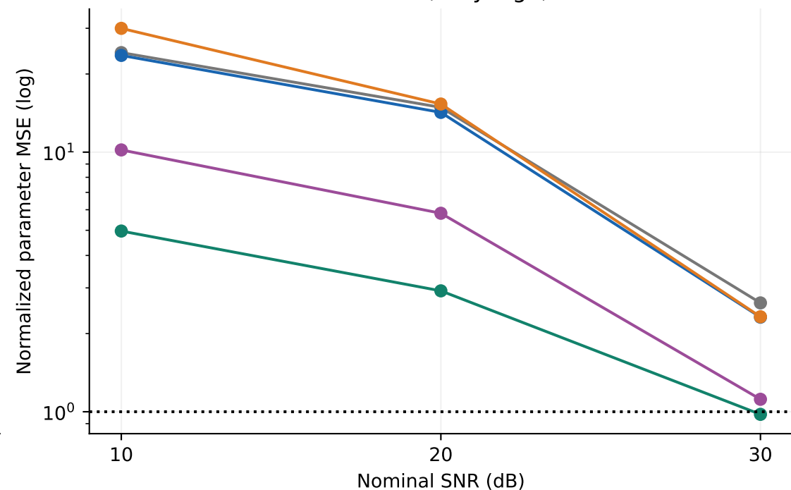
Primary condition: why full-H methods fail
