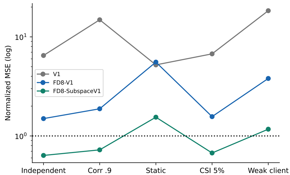
MNIST: limitations at 20dB
