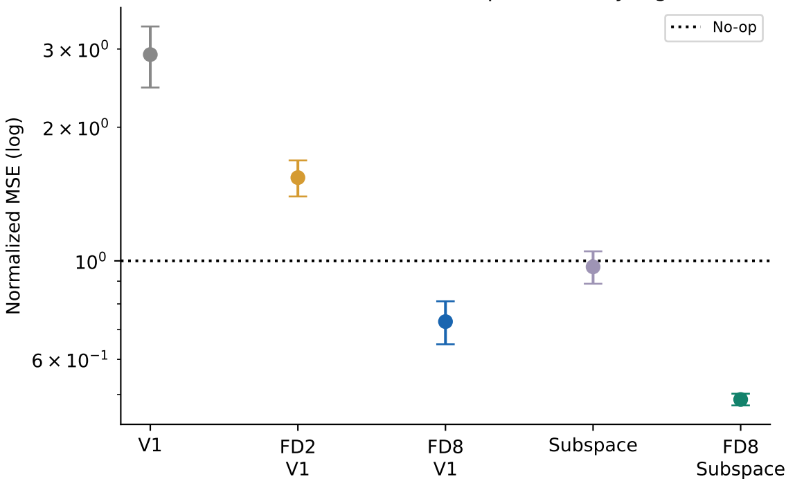
MNIST: limitations at 20dB
