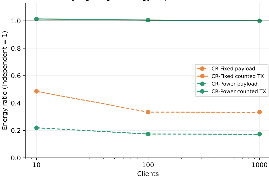
Rayleigh: signal energy vs protocol overhead
