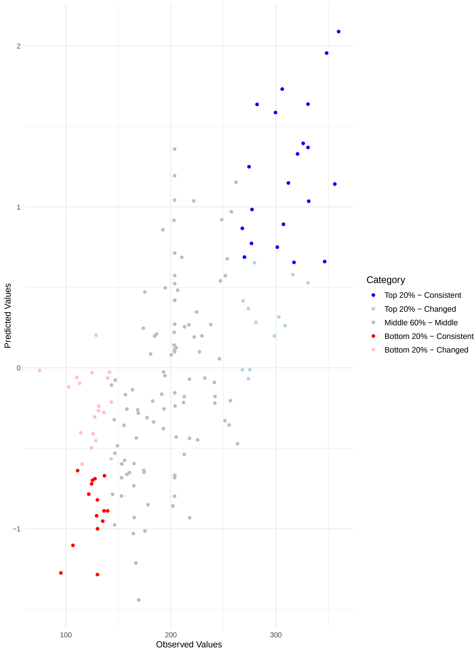
Comparing Predicted and Observed Rankings Across Validation Sets Kendall's Tau: 0.50 | Top 20% Consistency: 46.67% | Bottom 20% Consistency: 28.30%
