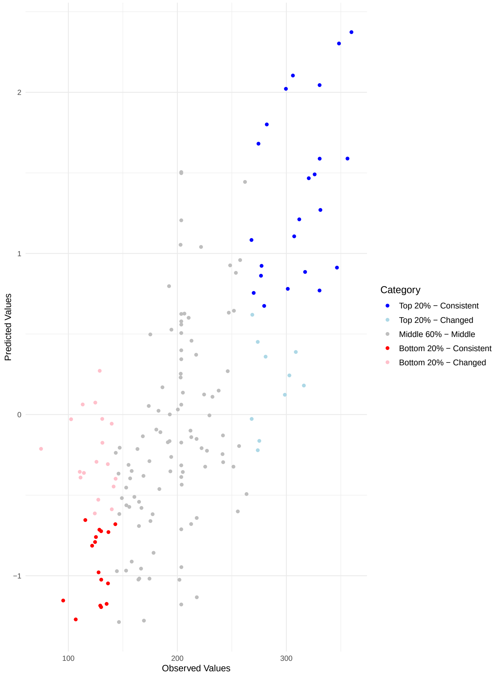
Comparing Predicted and Observed Rankings Across Validation Sets Kendall's Tau: 0.49 | Top 20% Consistency: 53.49% | Bottom 20% Consistency: 30.77%
