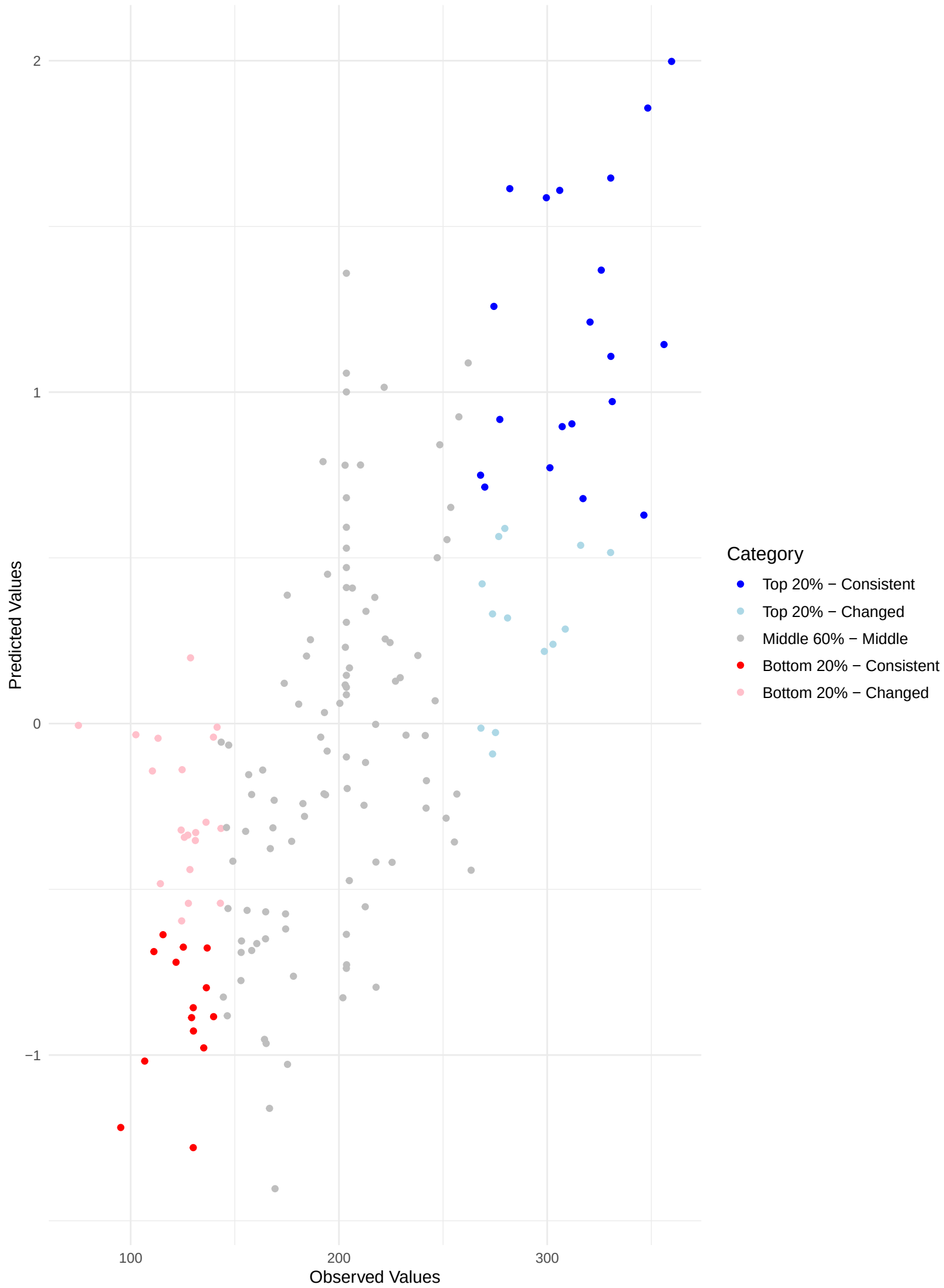
Comparing Predicted and Observed Rankings Across Validation Sets Kendall's Tau: 0.50 | Top 20% Consistency: 43.48% | Bottom 20% Consistency: 25.93%
