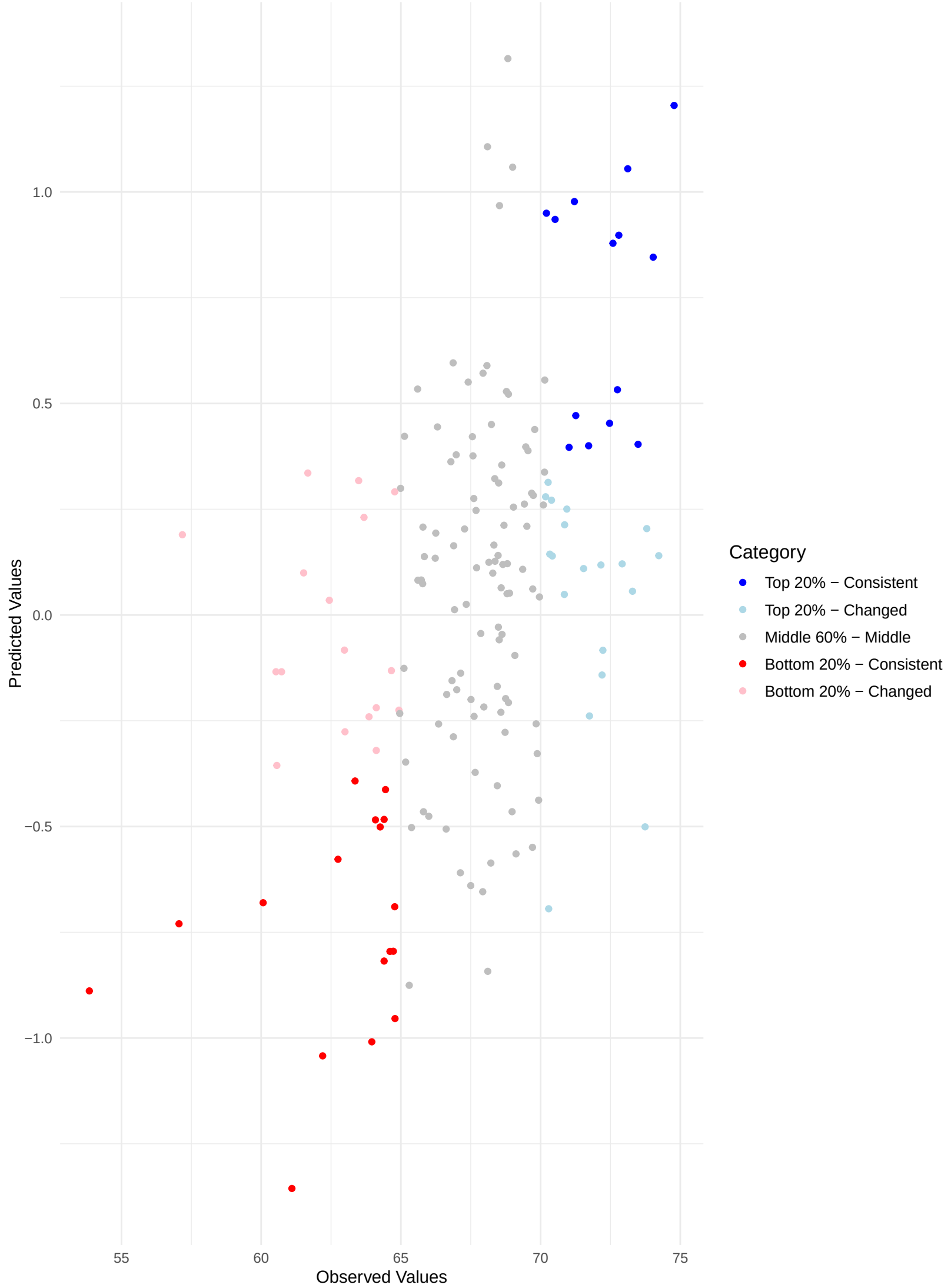
Comparing Predicted and Observed Rankings Across Validation Sets Kendall's Tau: 0.31 | Top 20% Consistency: 26.92% | Bottom 20% Consistency: 33.33%
