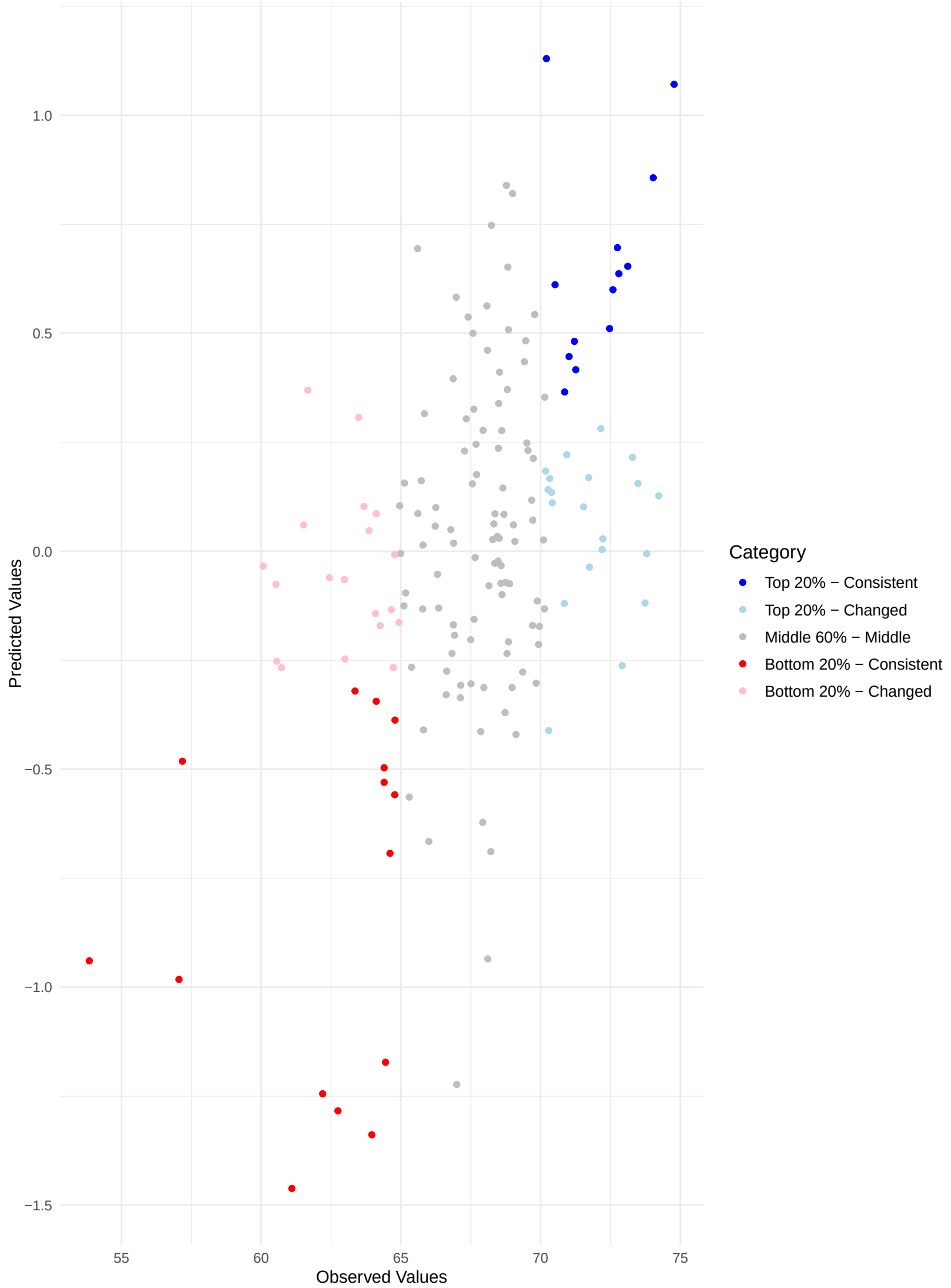
Comparing Predicted and Observed Rankings Across Validation Sets Kendall's Tau: 0.31 | Top 20% Consistency: 24.53% | Bottom 20% Consistency: 28.30%
