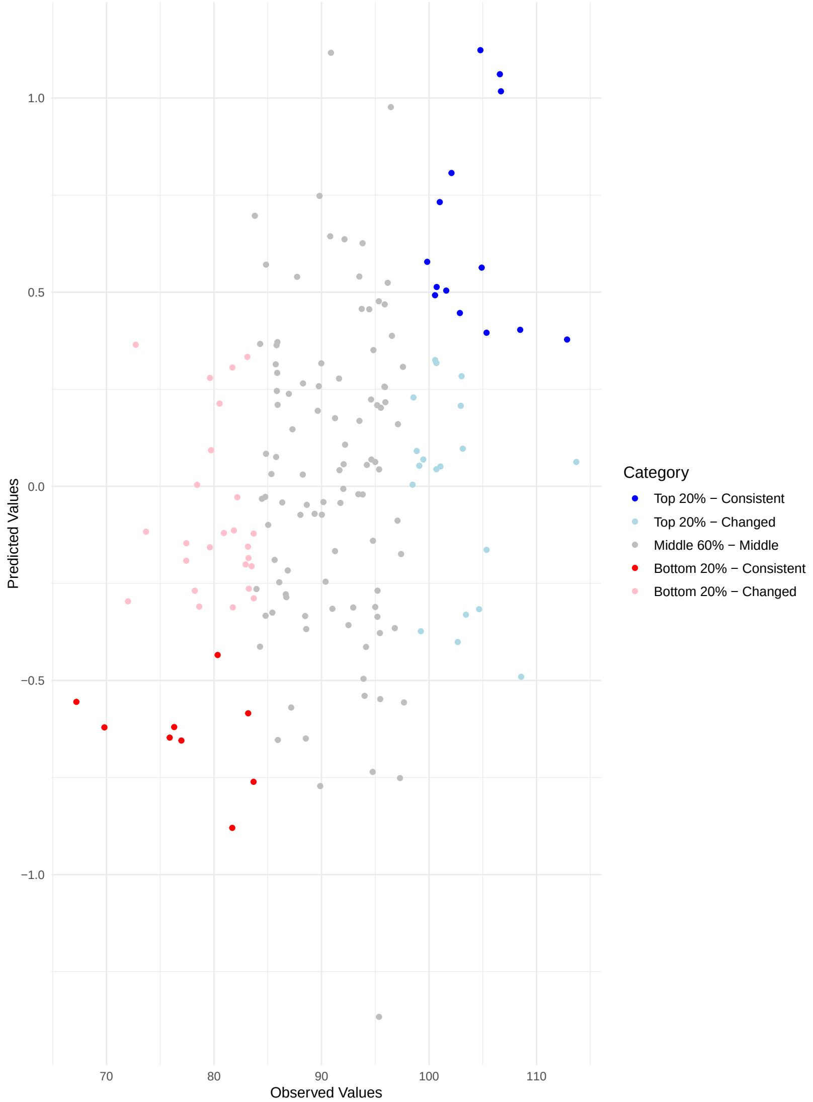
Comparing Predicted and Observed Rankings Across Validation Sets Kendall's Tau: 0.22 | Top 20% Consistency: 26.92% | Bottom 20% Consistency: 15.25%
