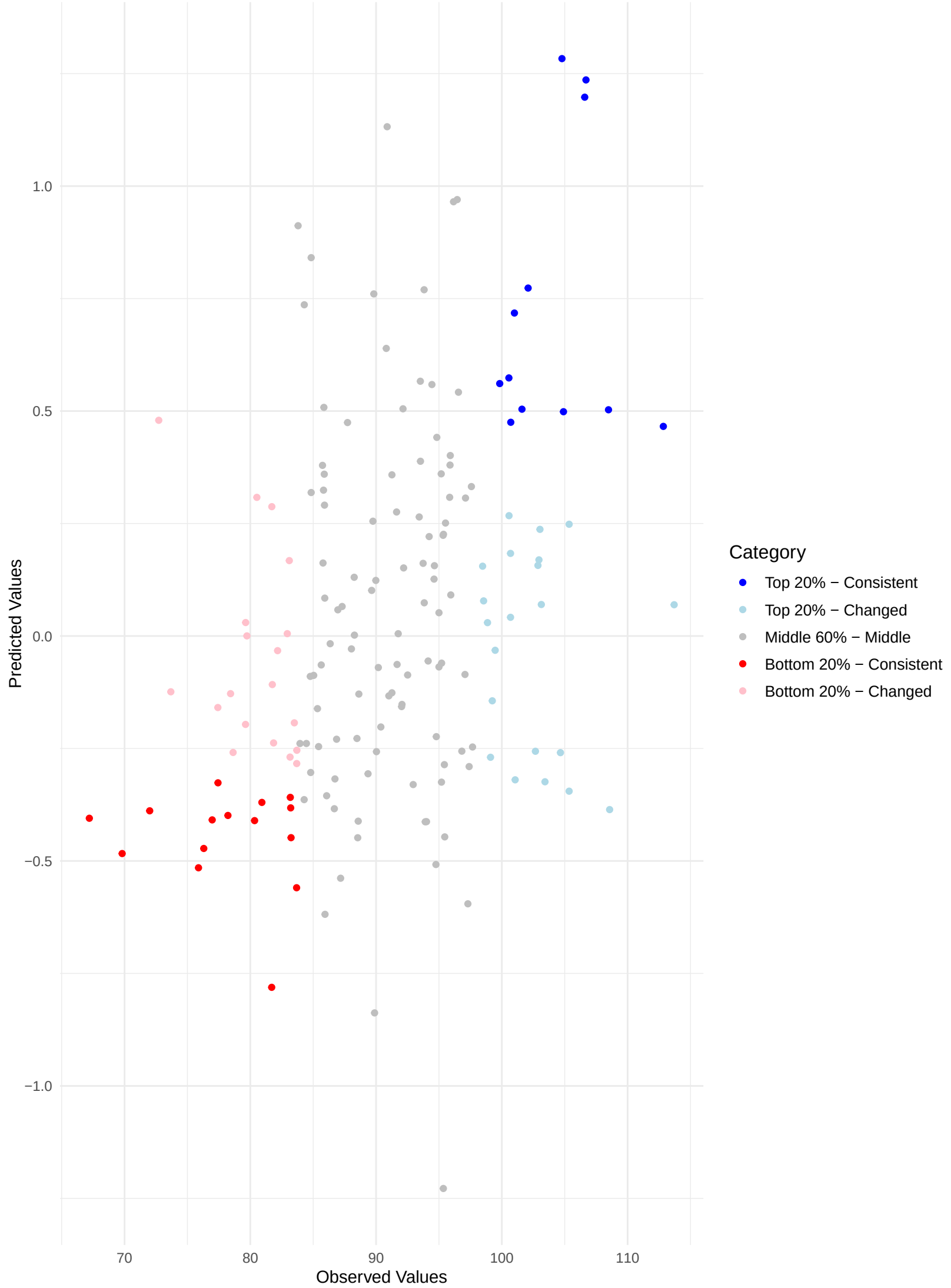
Comparing Predicted and Observed Rankings Across Validation Sets Kendall's Tau: 0.24 | Top 20% Consistency: 22.22% | Bottom 20% Consistency: 28.30%
