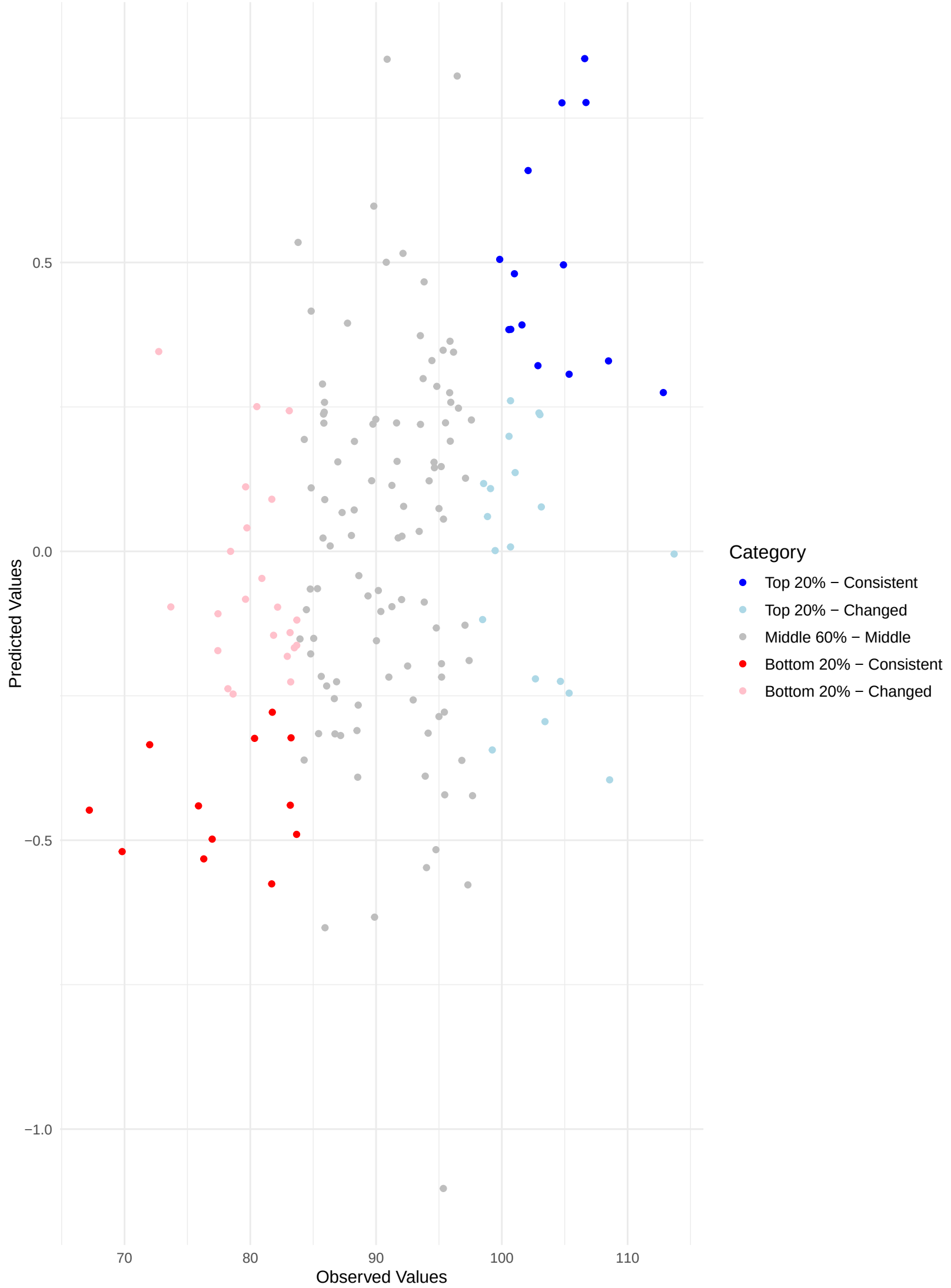
Comparing Predicted and Observed Rankings Across Validation Sets Kendall's Tau: 0.24 | Top 20% Consistency: 26.92% | Bottom 20% Consistency: 21.43%
